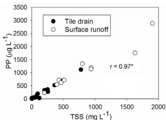
Fig. 3. Typical relationship between particulate P (PP) and total suspended sediment (TSS) in water sampled from tile drains and surface runoff. Data were collected from Field 8 in the Ewing subwatershed (Quebec, Canada). *Significant at the 0.05 probability level.
