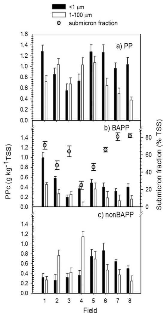
Fig. 6. Mean (a) particulate P (PP), b) bioavailable particulate P (BAPP), and (c) nonbioavailable particulate P (non-BAPP) concentrations in submicron material (<1 µm) and micrometric material (1–100 µm) of total suspended sediments (TSS) from eight agricultural fields (Ewing subwatershed, Quebec Canada). Data points on (b) are the mean submicron contribution to TSS for each field. The bars on each column and data points are the standard errors of the mean.
